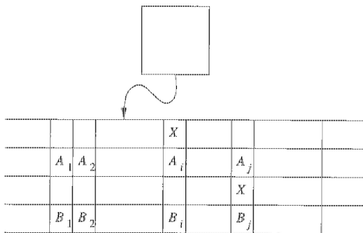
Figure 8.17: Simulation of a two-tape Turing machine by a one-tape Turing
