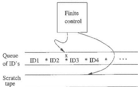
Figure 8.18: Simulation of an NTM by a DTM
